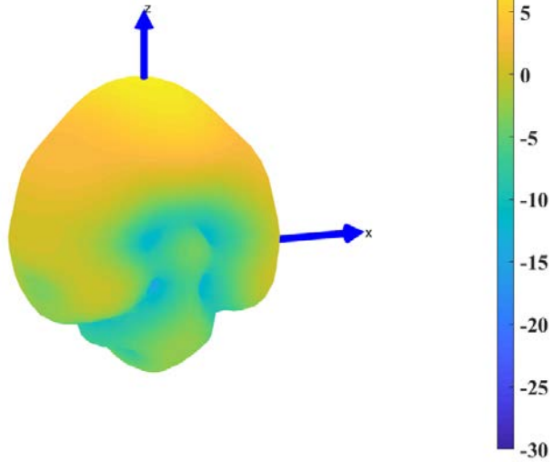
Realized gain, f = 2 GHz
